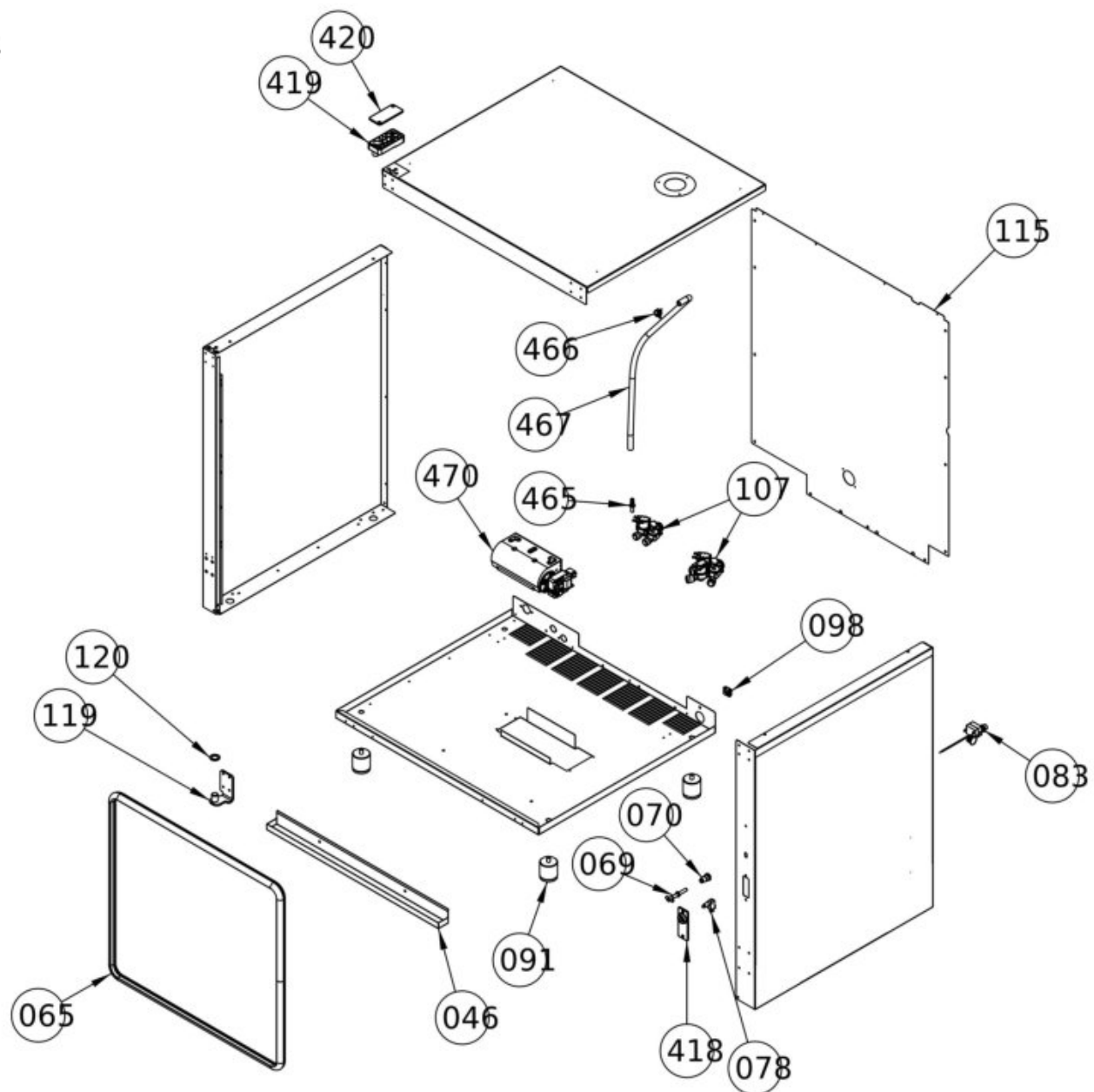
Oven body
