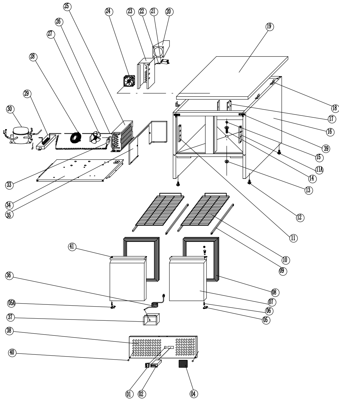
E-G-SS45BT EXPLODE
